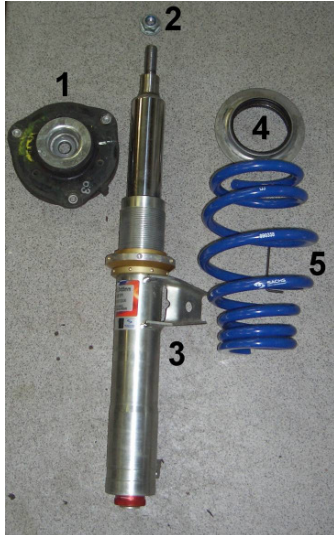
Front Axle
