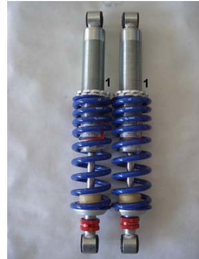
Rear Axle
